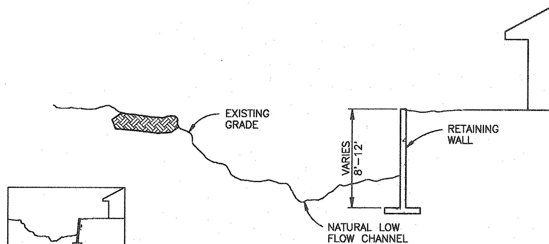
HIGH ERODING BANK STABILIZATION
