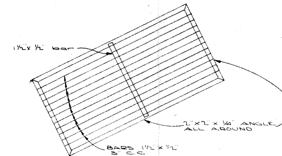
STEEL TRASH RACK DETAILS
