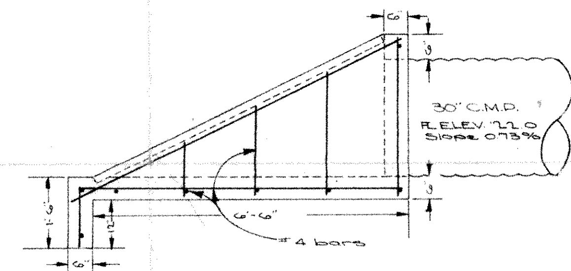
DRAIN INLET DETAILS
