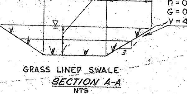
GRASS LINED SWALE SECTION A-A
